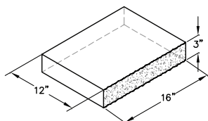
ISOMETRIC VIEW 3" RECTANGULAR CAP
