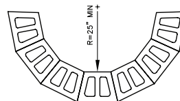
OUTSIDE RADIUS DETAIL NICOLOCK WALL
