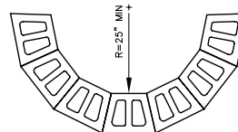
OUTSIDE RADIUS DETAIL NICOLOCK WALL
