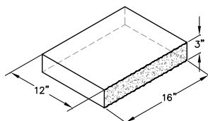
ISOMETRIC VIEW 3" RECTANGULAR CAP
