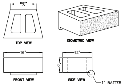
WALL UNITS (6"x16" UNIT)
