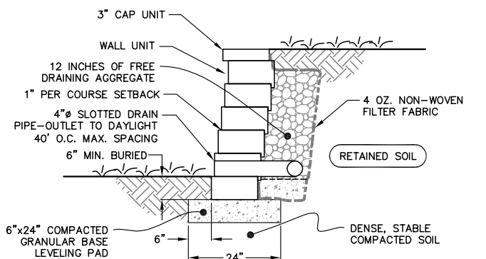
NICOLOCK WALL — TYPICAL GRAVITY CROSS SECTION
